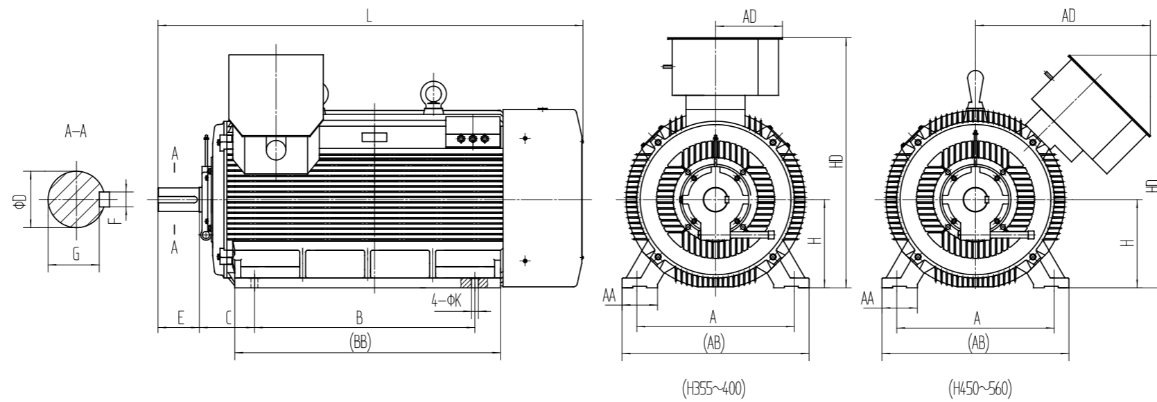
YPT-400-450 安装尺寸表 (690V, IC416) YPT400-450 MOUNTING DIMENSIONS TABLE (690V, IC416)
